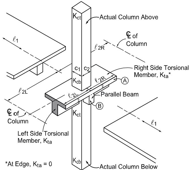
Figure 2-8 Equivalent column
