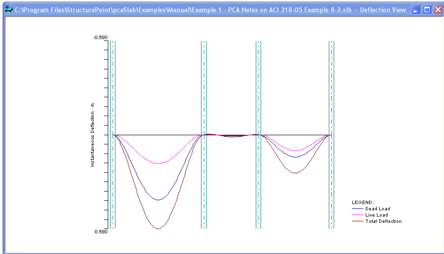
Figure 4-87 View Deflection Diagram
