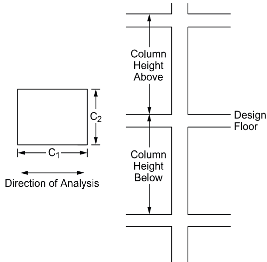
Figure 4-24 Required Column Dimensions
