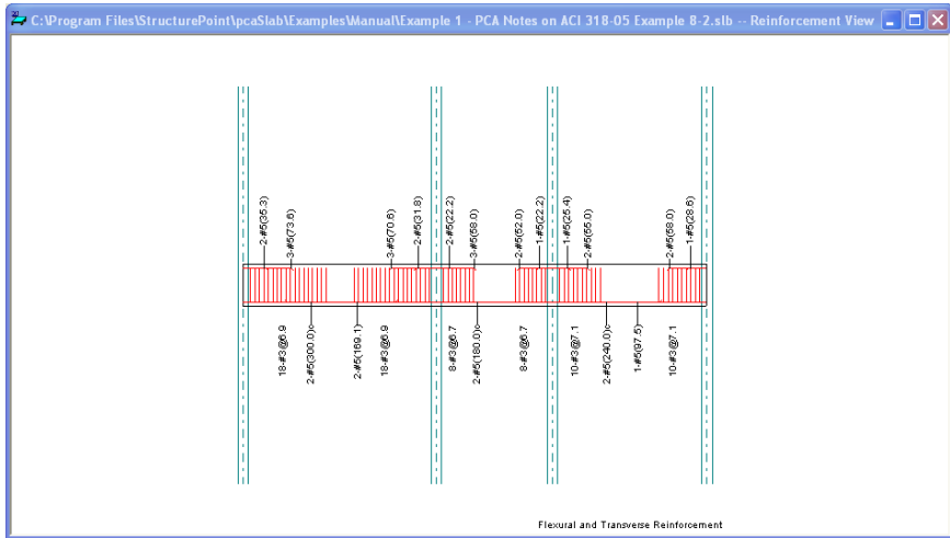
Figure 4-85 View Reinforcement
