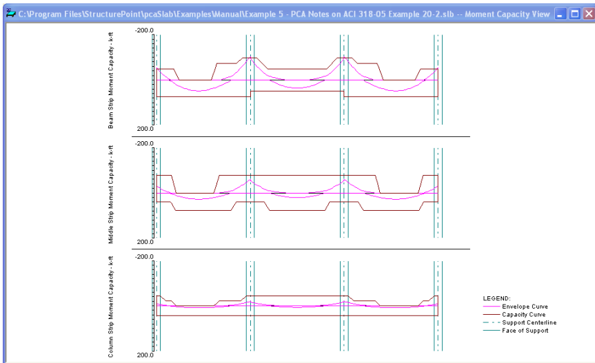
Figure 4-81 View Moment Capacity Diagram
