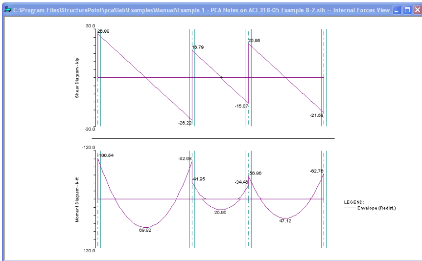
Figure 4-78 View Internal Forces Diagram
