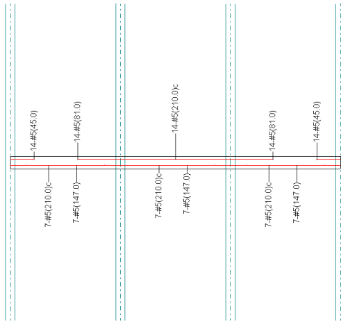
Middle Strip Flexural Reinforcement
