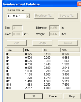
Figure 4-96 Changing Reinforcement Database
