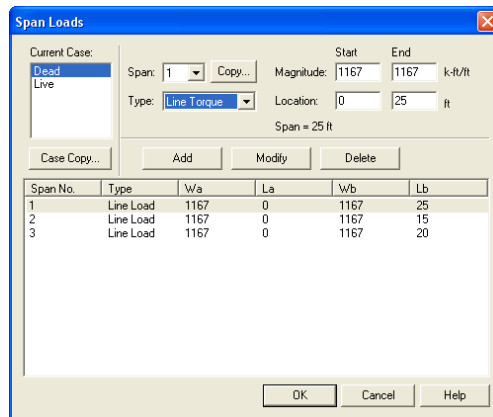
Figure 4-53 Defining Line Torque on Span
