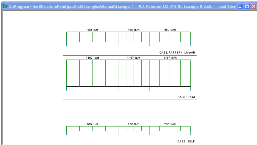
Figure 4-75 Loads View Window
