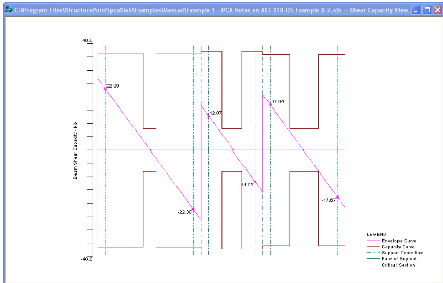
Figure 4-83 View Shear Capacity
