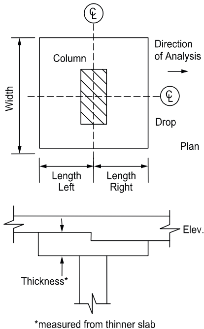
Figure 4-26 Required Drop Dimensions
