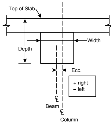
Figure 4-30 Required Transverse Beam Dimensions
